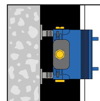
In-front-of-wall installation.
