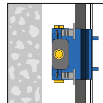
Installation on prefabricated cells.
