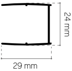
profilo murale profilé mural_wall profile
