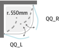
SOHO QQ chiusura semicircolare porte quart de rond quarter-round enclosure
