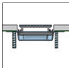
Flat Cover aluminium + stainless steel
