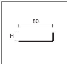
CPLB/2 punched base for tiled floors
