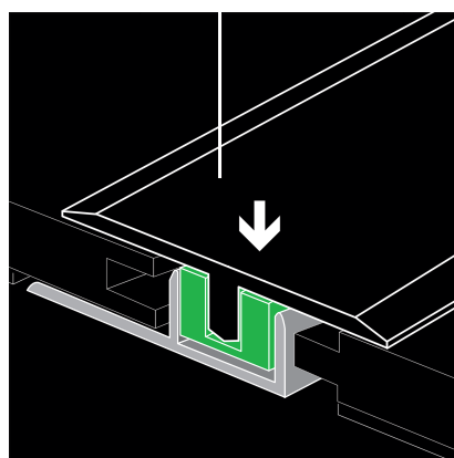
push the top profile in the base
