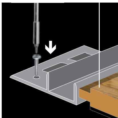
fix the aluminium base to the subfloor with screws or glue
