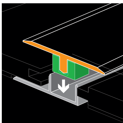
put the top profile in the base
