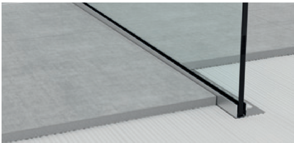
GPS1/DX/19 satin stainless steel AISI 304 DIN 1.4301
