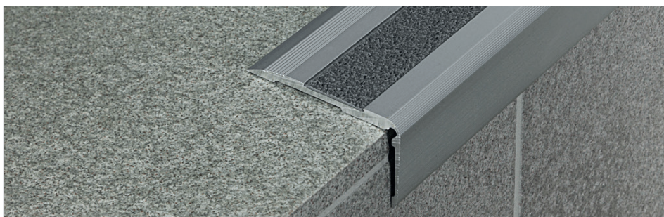
76/F silver anodised aluminium + black slip-resistant insert
