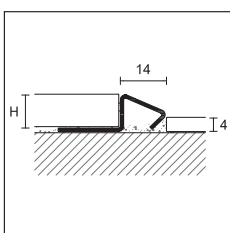
MIN/10 application for floors of different height
