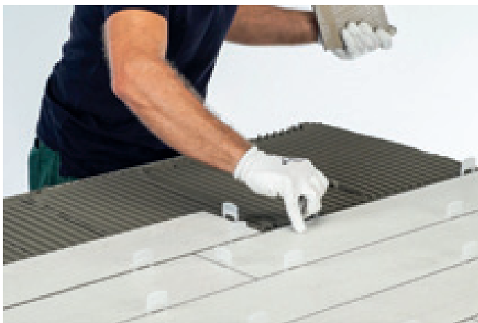
disposable clips installation
